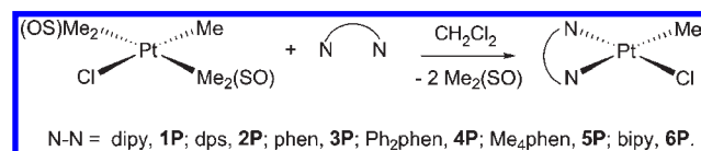
Scheme 2. Synthetic Pathway to Methyl Chloride Platinum(II) Complexes 1P – 6P
