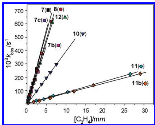
Figure 4. Dependence of the observed pseudo-first-order rate constants ( k_{\text{obs}}/\text{s}^{-1} ) for ethene exchange on complexes 7 , 8 , and 10–12 as a function of different amounts of free ethylene (experimental conditions: C_{\text{Pt}} = 3\text{--}5\text{ mm} , [\text{C}_2\text{H}_4] = 0\text{--}30\text{ mm} in chloroform- d at 298 K).
