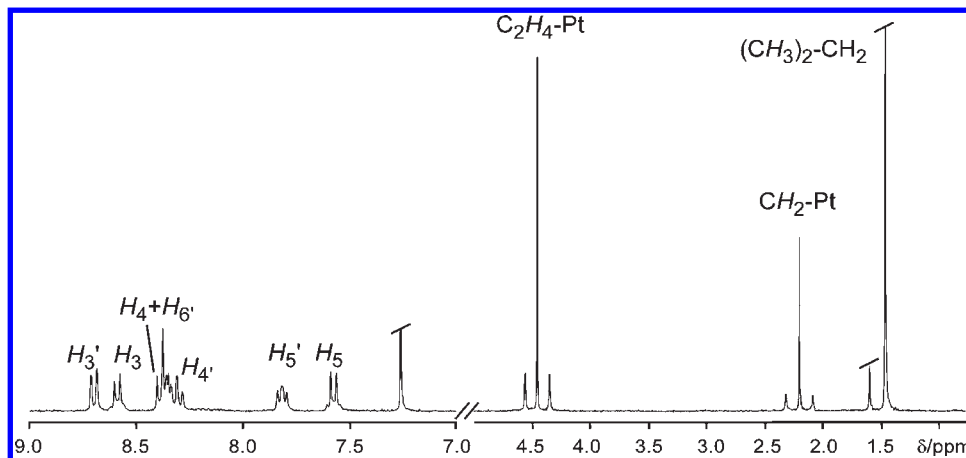
Figure 2. ^1\text{H} NMR spectrum of complex 7b recorded at 300.13 MHz in chloroform- d at 298 K.
