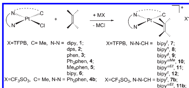
Scheme 3. Synthetic Pathway to Uncyclometalated ( 1–6 ) and Cyclometalated ( 7–12 ) Platinum(II) Ethene Complexes a
