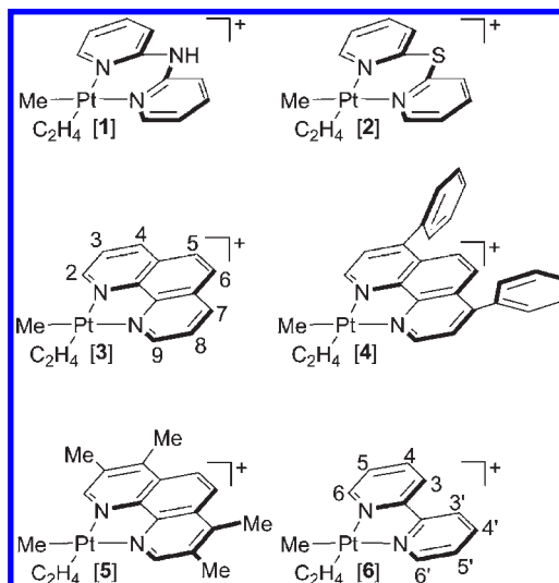
Chart 1. Structural Formulas for the Complexes 1–6 , with the Numbering Scheme
