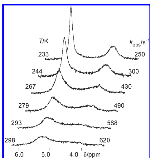
Figure 5. Variable-temperature ^1\text{H} NMR spectra of complex 8 showing the free and coordinated ethylene protons peaks (chloroform- d ; 300.13 MHz; experimental conditions: C_{\text{Pt}} = 3.55\text{ mm} ; [\text{C}_2\text{H}_4] = 6.26\text{ mm} ; temperature, T/\text{K} , and rate constants, k_{\text{obs}}/\text{s}^{-1} , for the ethene exchange are reported on the left and the right side of the spectra, respectively).
