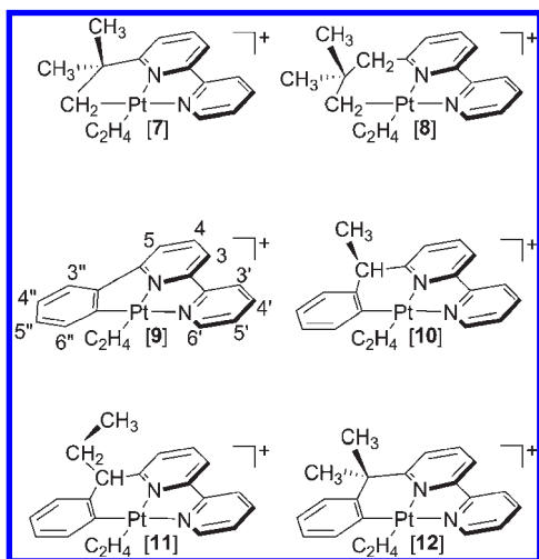
Chart 2. Structural Formulas for the Complexes 7–12, Together with the Adopted Numbering Scheme
