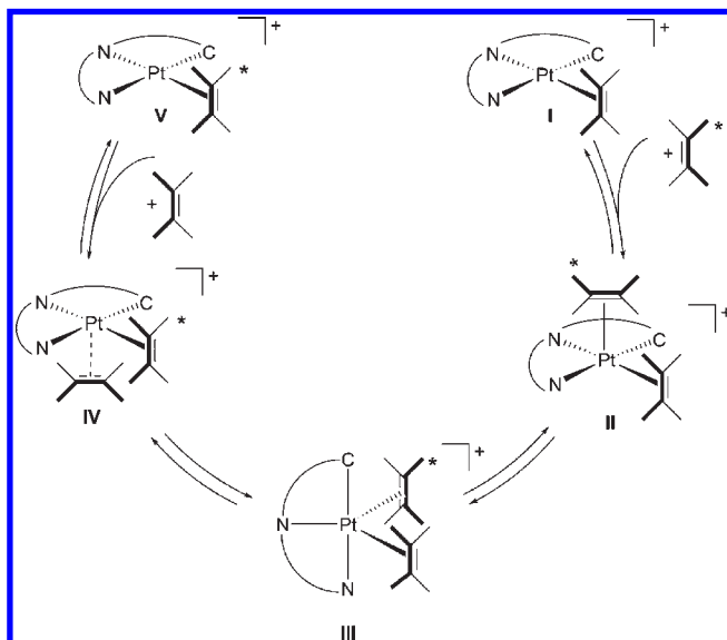
Scheme 6. Associative Mechanism for the Ethene Exchange on Square-Planar Cyclometalated Platinum(II) Species 7–12 in Chloroform- d Solutions
