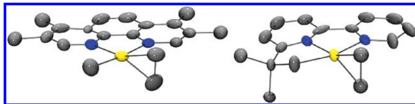
Figure 1. ORTEP view for the platinum(II) cationic complexes 5 and 7 .
