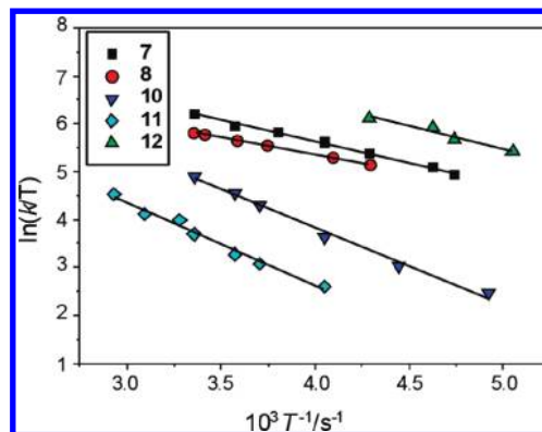
Figure 6. Eyring plots obtained for ethene exchange on cyclometalated platinum(II) complexes 7 , 8 , and 10–12 from ^1\text{H} DNMR data measured in chloroform- d .
