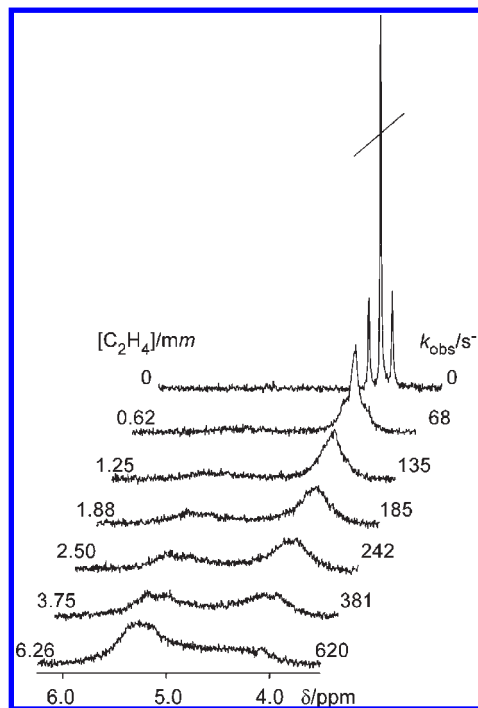
Figure 3. Aliphatic portion of the ^1\text{H} NMR spectra of 8 showing the line-broadening effect on the signal of the coordinated olefin as a function of ethene concentration (chloroform- d ; 300.13 MHz; experimental conditions: T = 298 K; C_{\text{Pt}} = 3.55 mM; ligand concentrations, [\text{C}_2\text{H}_4]/\text{mm} , and best-fit first-order rate constants, k_{\text{obs}}/\text{s}^{-1} , for the ethene exchange are reported on the left and the right side of the spectra, respectively).
